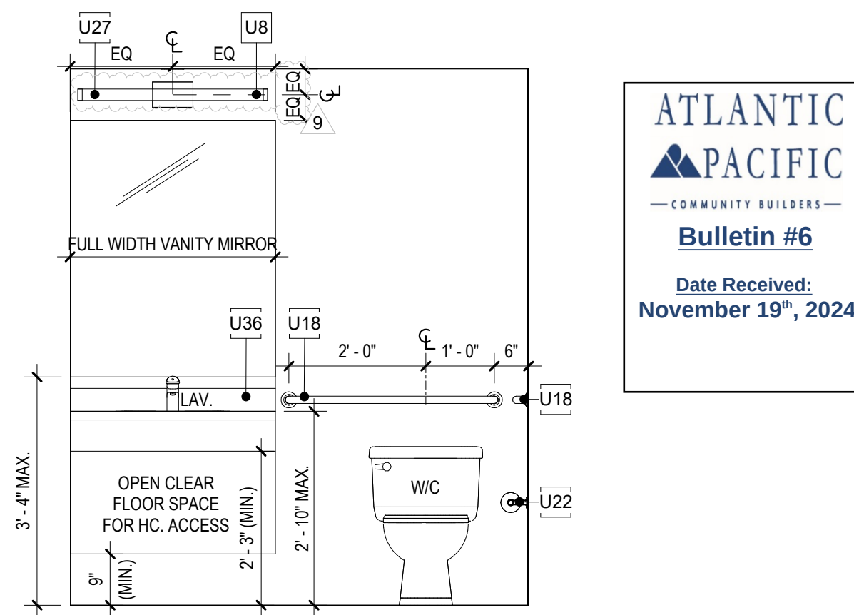
UNIT A2 FA BATHROOM EL. SCALE: 1/2" = 1'-0"
