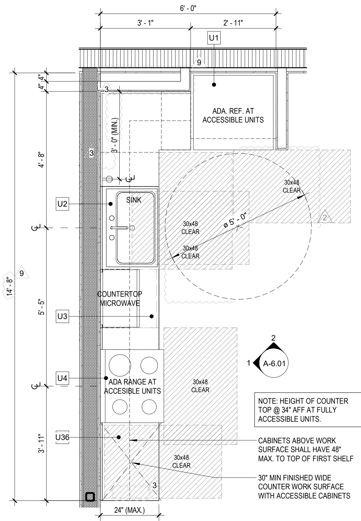
UNIT A2 FA KITCHEN PLAN SCALE: 1/2" = 1'-0"
