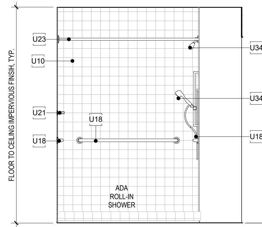
UNIT A2 FA BATHROOM EL. SCALE: 1/2" = 1'-0"
