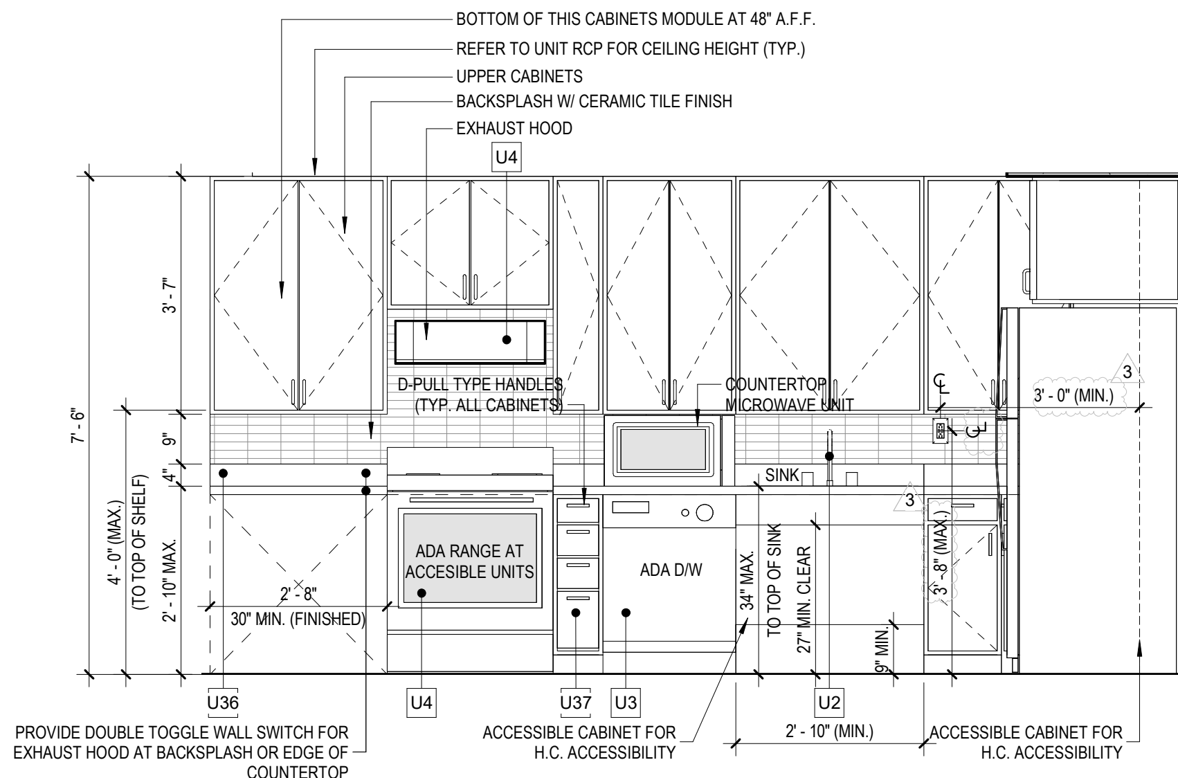
UNIT A2 FA KITCHEN EL. SCALE: 1/2" = 1'-0"
