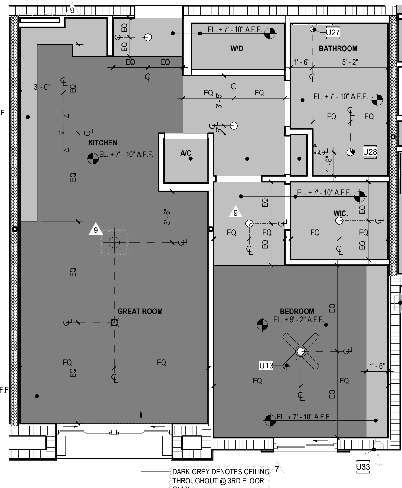
UNIT A2 FULLY ACCESSIBLE RCP SCALE: 1/4" = 1'-0"
