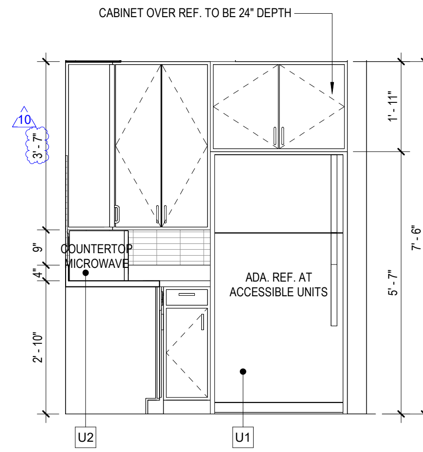
UNIT A1 KITCHEN EL. SCALE: 1/2" = 1'-0"
