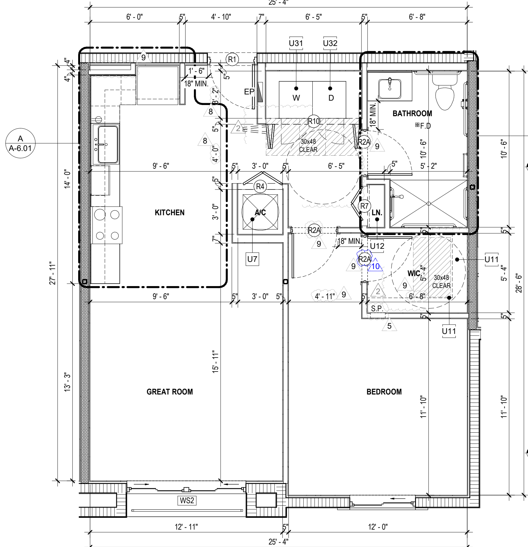
UNIT A2 FULLY ACCESSIBLE FLOOR PLAN SCALE: 1/4" = 1'-0"
